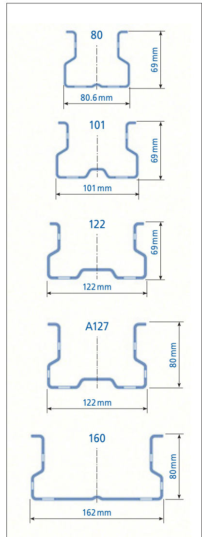
Figure 8. Uprights used
